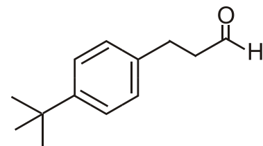
4-(1,1-dimethylethyl)-benzene propanal
